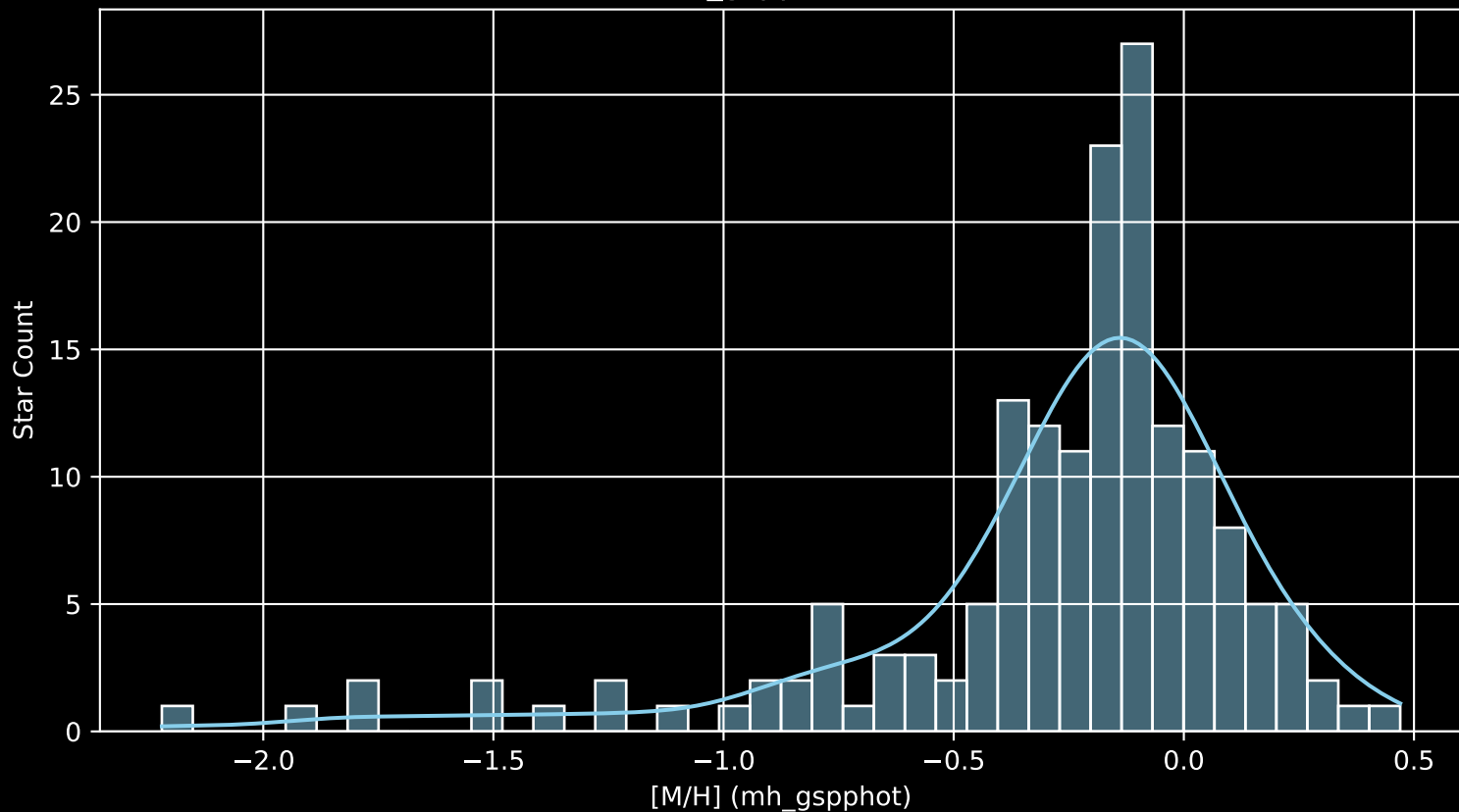
APOGEE DR17 Field: [116+04 [M/H] (mh_gspphot) (n= 165)
