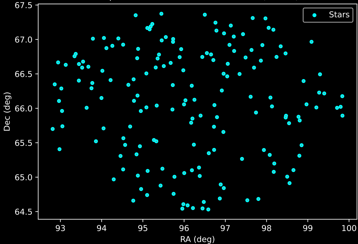
APOGEE DR17 Field: [116+04] Proper Motion Vectors for Gaia Star Field (n= 169)
