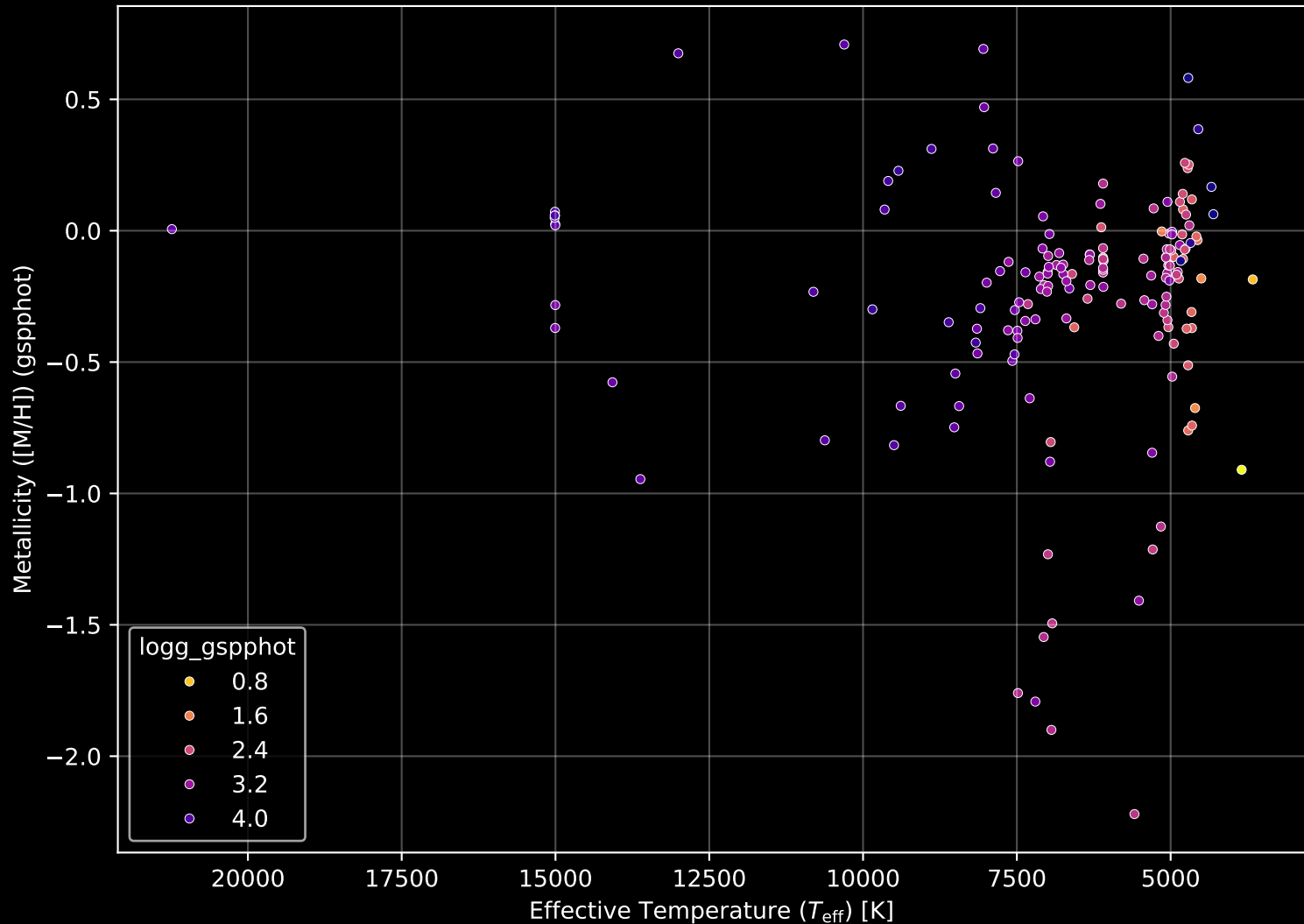
APOGEE DR17 Field: [116+04] Stellar Population Parameters (n= 169)
