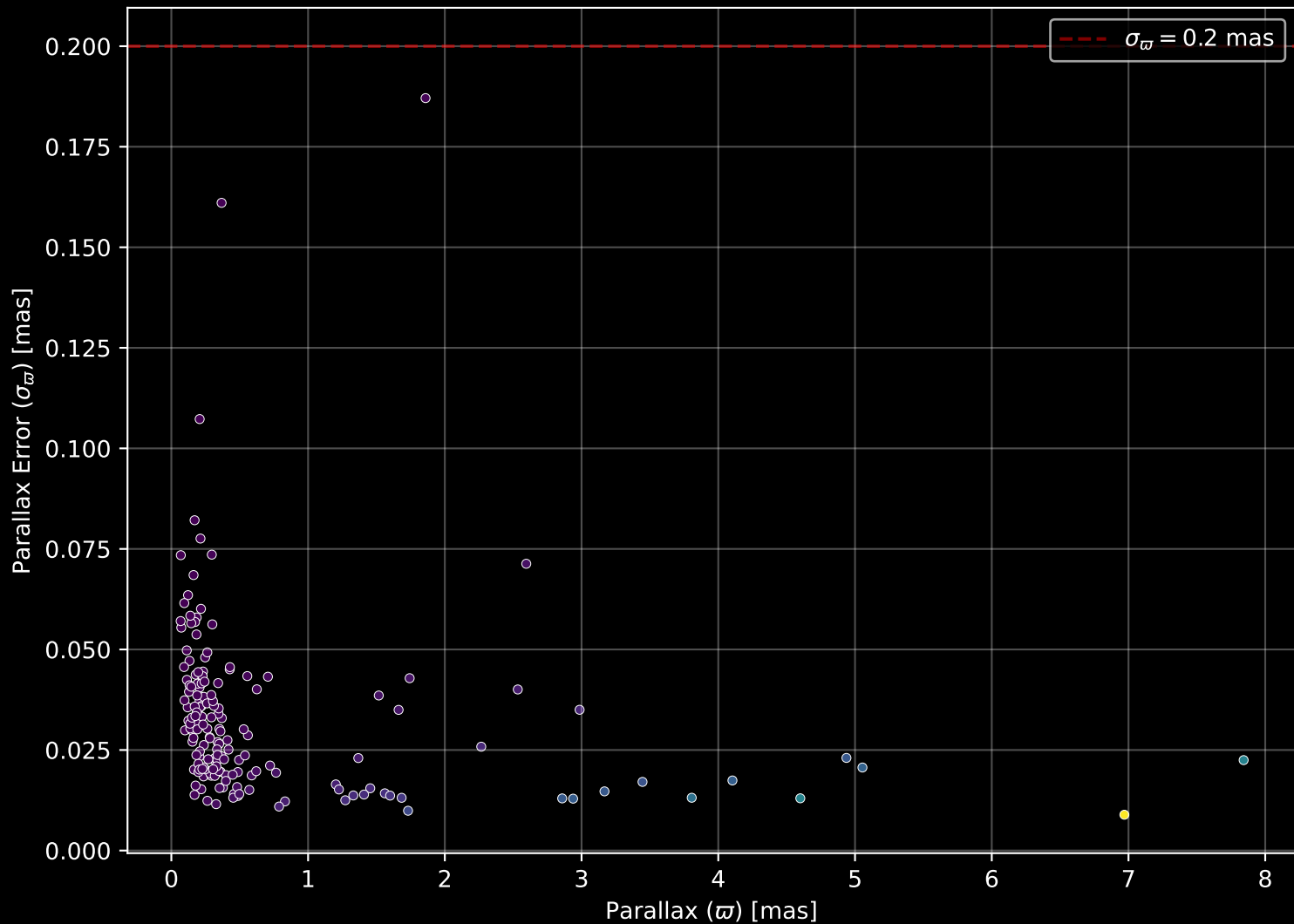
APOGEE DR17 Field: [116+04] Parallax Quality (n= 169)
