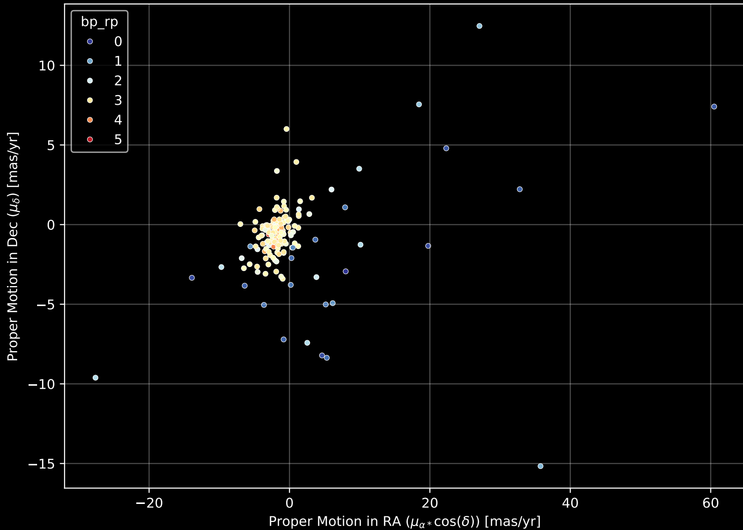
APOGEE DR17 Field: [116+04] Proper Motion Diagram (n= 169)
