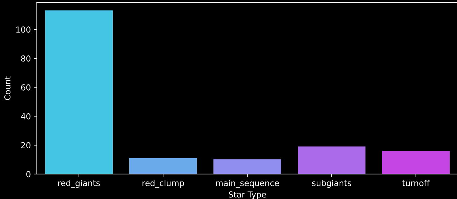
APOGEE DR17 Field: [116+04] Count plot of Star Type
