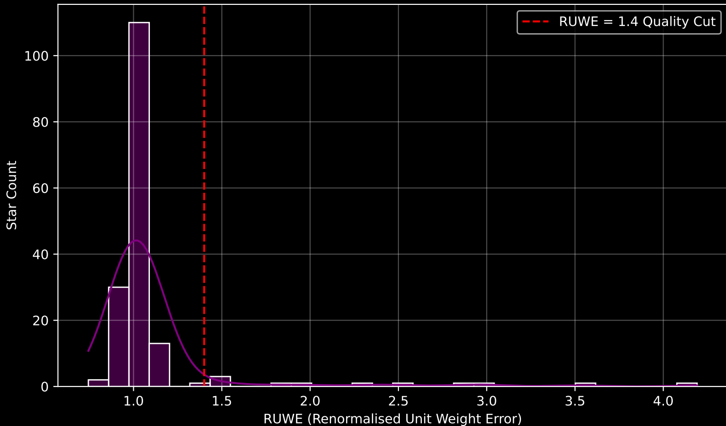
GAPOGEE DR17 Field [116+04] RUWE Distribution (n= 167)
